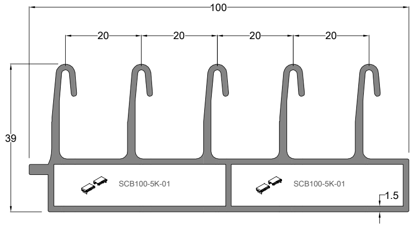
5 Raylı Eşikli Alt Ray Profili BOTTOM QUINTUPLE RAIL PROFILE (THRESHOLD)
