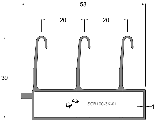
3 Raylı Eşikli Alt Ray Profili BOTTOM TRIPLE RAIL PROFILE (THRESHOLD)
