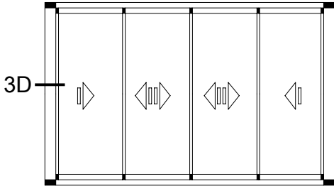
4. Kilit Alternatifi : Kanca Kilitli Detay LOCK ALTERNATIVE : HOOK LOCKED DETAIL
