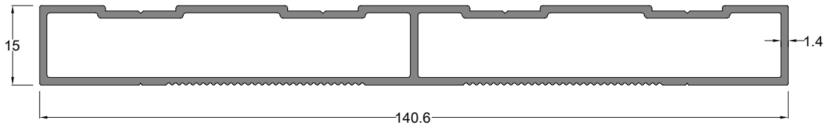
4 Raylı Yan Kasa Profili QUAD RAIL FRAME PROFILE (SIDE)
