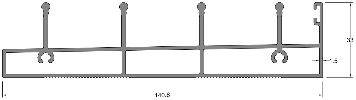
4 Raylı Eşikli Alt-Üst Ray Profili QUAD RAIL THRESHOLD PROFILE (BOTTOM-TOP)
